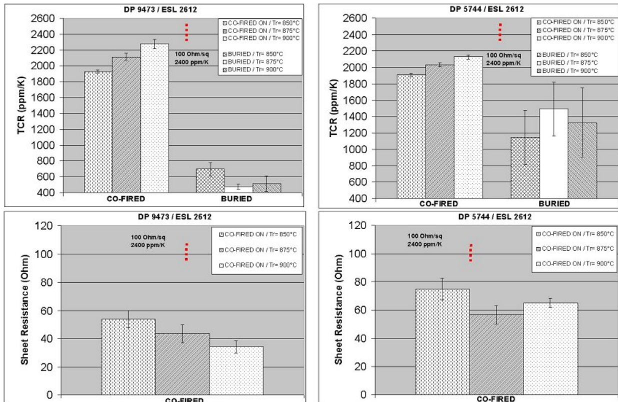
Fig. 2. TCR and SR at different processing conditions for Ag (left column) and Au conductors. For SR, only values of co-fired resistors are presented
