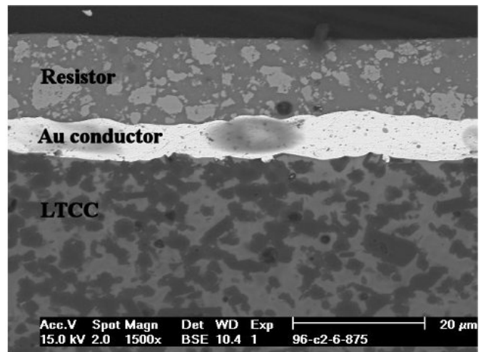
Fig. 6. Dilatometry analysis of the tape and the conductors used (left). Au expands starting from 700°C, which is around the onset temperature for the tape shrinkage. Au conductor on a co-fired resistor – tape system (right)
