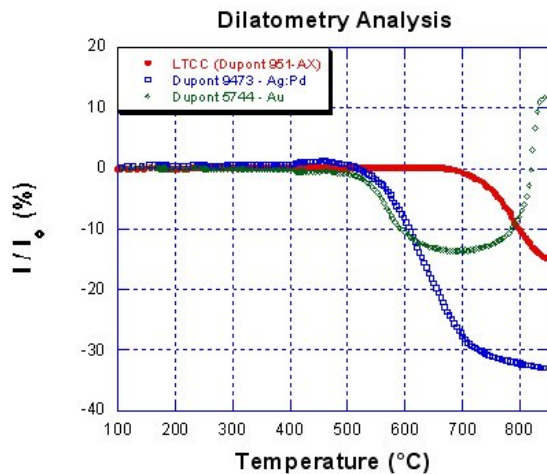
Fig. 6. Dilatometry analysis of the tape and the conductors used (left). Au expands starting from 700°C, which is around the onset temperature for the tape shrinkage. Au conductor on a co-fired resistor – tape system (right)
