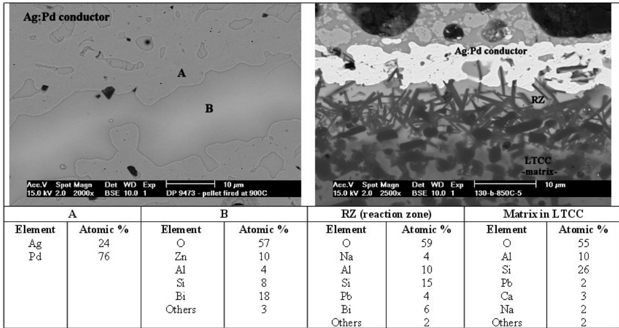
Fig. 5. EDXS analysis of Ag pellet (left) and RZ-reaction zone (light grey) and LTCC matrix (dark grey). RZ contains glass species from both LTCC matrix and the conductor. Image on the right is an LTCC structure fired at 850°C
